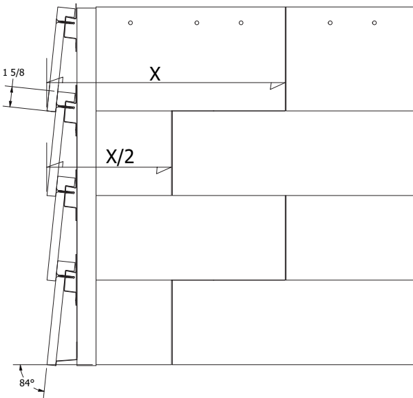
L Shape External Corner Assembly
