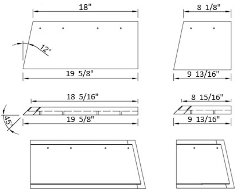
Corner Detail Cutting Guide for U Shape
