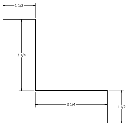
Internal Corner Trim
