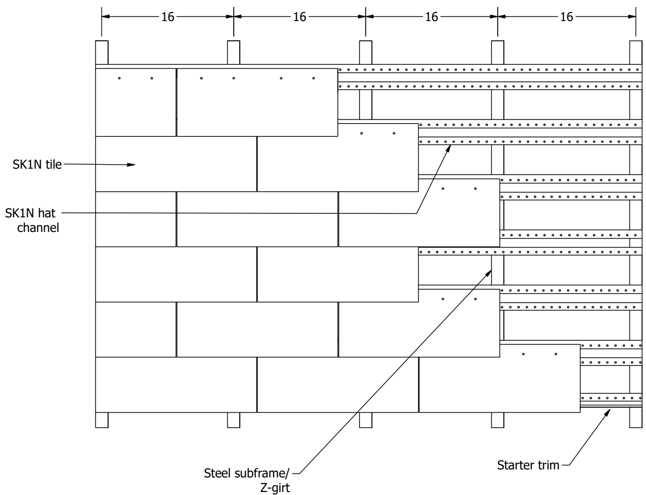
Elevation of SK1N System
