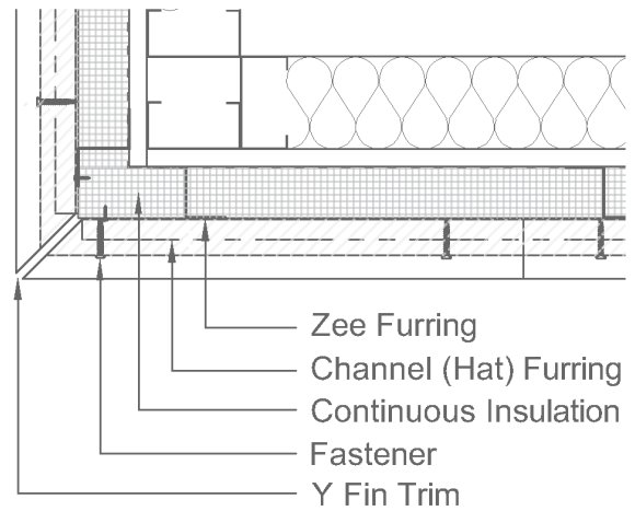
Mitred External Corner with Y Fin Trim
