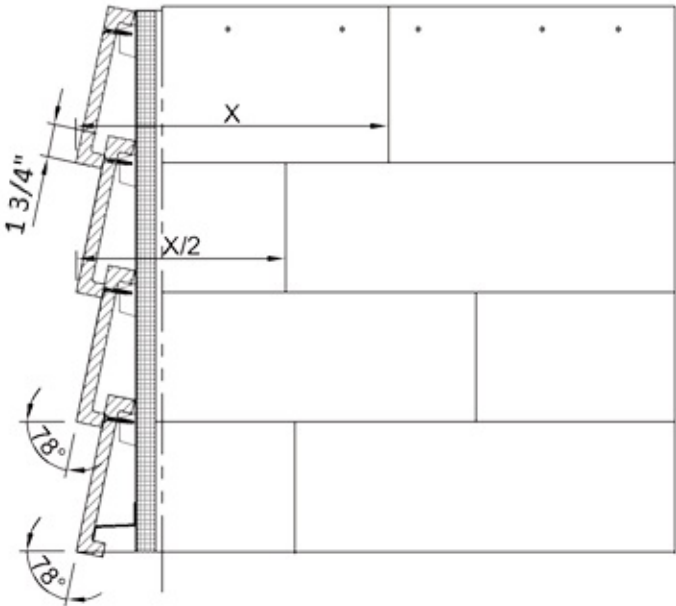
U Shape External Corner Assembly
