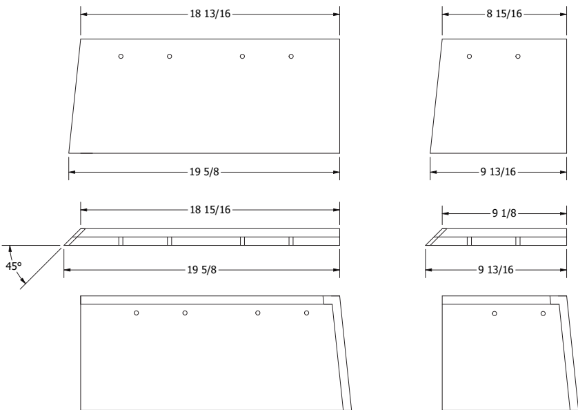
Corner Detail Cutting Guide for L Shape
