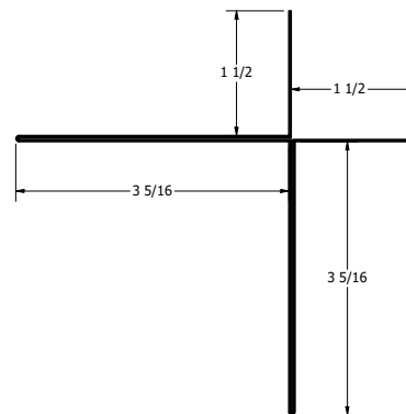
Inwards External Corner Trim
