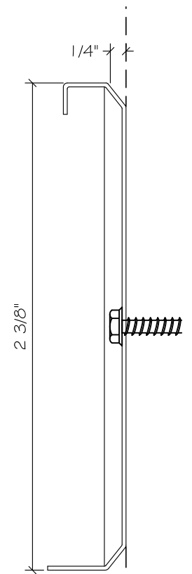
SECTION OFFSET RIBS
