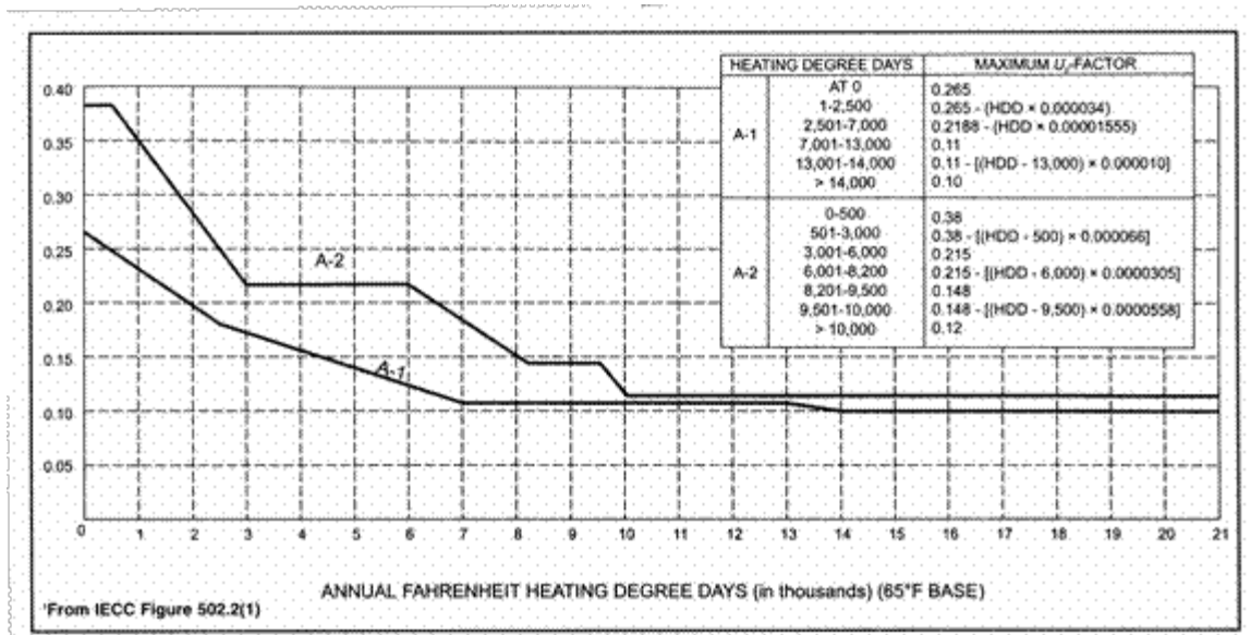
U_o Walls—Type A-1 and A-2 Residential Buildings—Heating'
