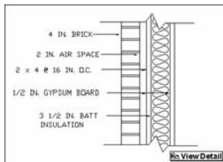
(a) 4 IN. BRICK AND WOOD STUD WALL
